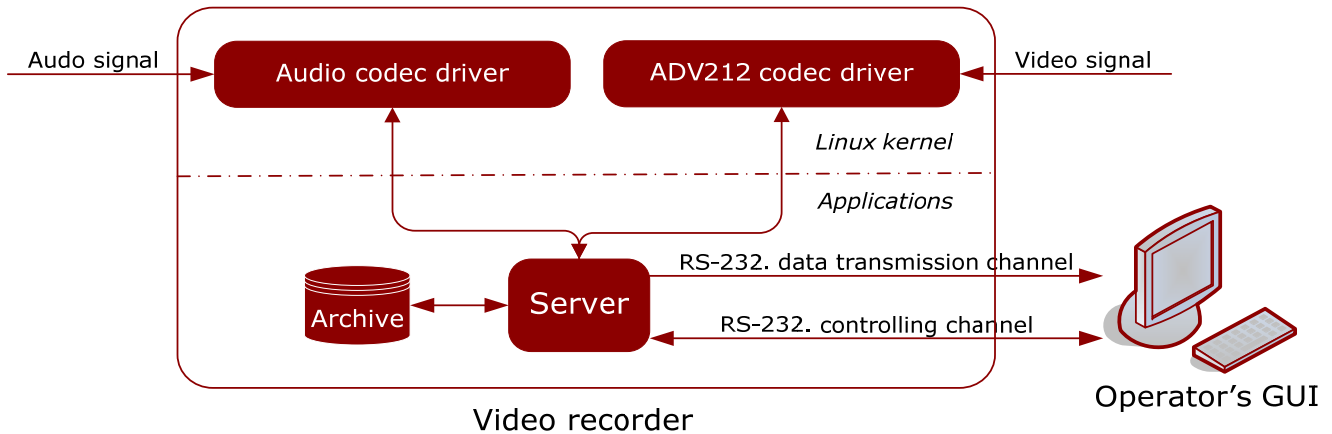
Figure 2. Block diagram of video registration device
