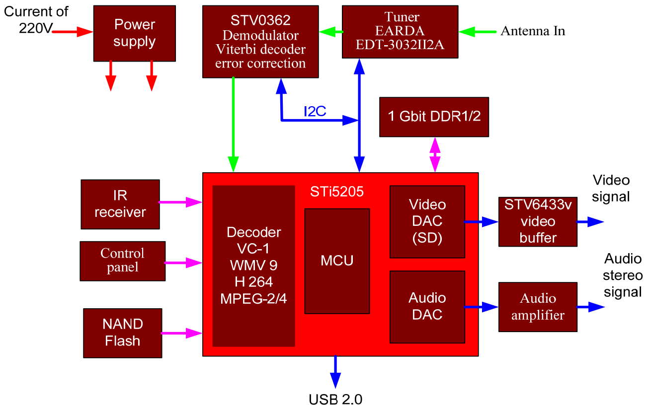
Figure 2. Layout of the structure of the device
