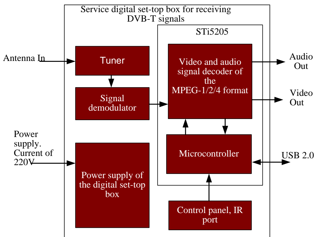
Figure 1. General structure of the device
